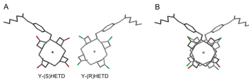
Figure 8. Noncoordinating carboxylate oxygen atoms of Y-(S)HETD and Y-(R)HETD are colored red and green, respectively, and are important for binding to antibody 2D12.5. Although these two molecules are enantiomers, the nature of the metal-complexed DOTA moiety allows for the two molecules and their noncoordinating carboxylate oxygen atoms to be almost superimposed.
