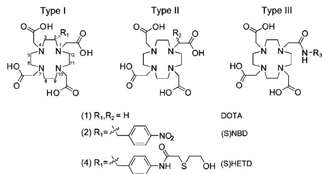
Figure 1. DOTA analogues used as probes, 15 showing sites of attachment to other molecules ( R_1 , R_2 , R_3 ). Type I analogues bind to antibody 2D12.5; the S enantiomer binds more tightly than the R enantiomer.
