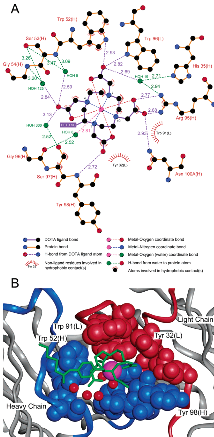
Figure 6. (A) Diagram showing the principal contacts between antibody and haptin in the 2D12.5–Y-(S)HETD complex, including five crystallographic water molecules. The Gd-(S)NBD is very similar. Figure was designed with the aid of Ligplot. 44 (B) Three-dimensional structure showing the crystallographic bridging water molecules and the protein side chains within 5 Å of the Y-(S)HETD. Figure was prepared with InsightII (Accelrys).
